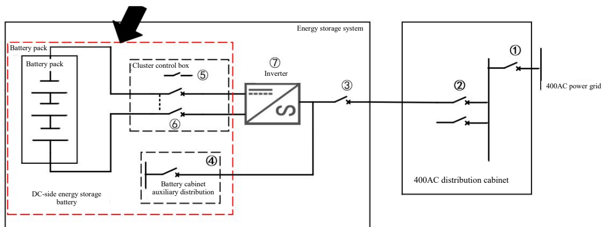
Figure 7.2.1 Power-on process
