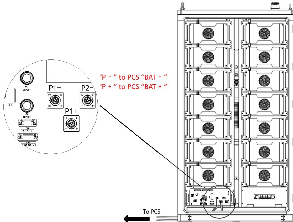
Figure 6.6 PCS Connection Diagram
