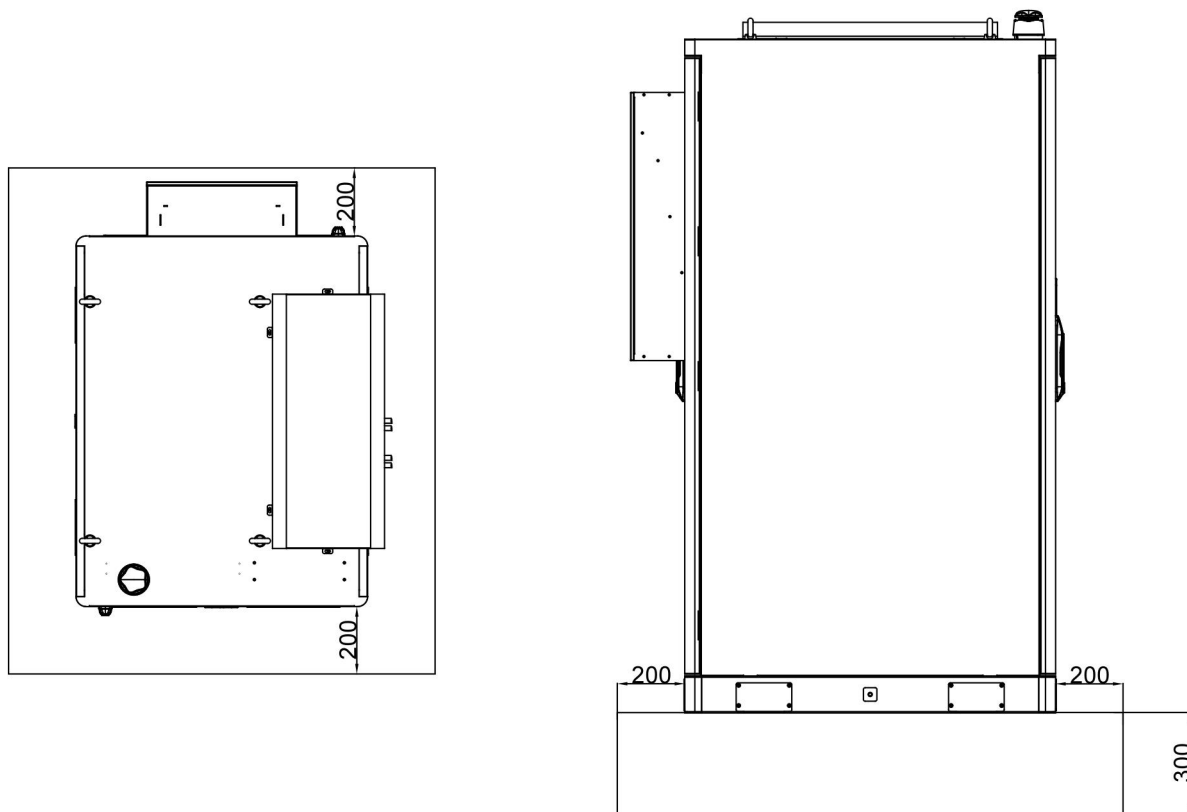
Figure 5.3 Schematic diagram of foundation installation
