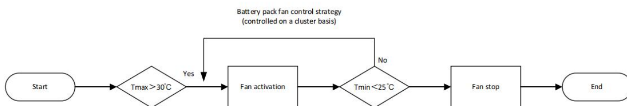
Figure 2.5.2 Battery Pack Fan Control Logic
