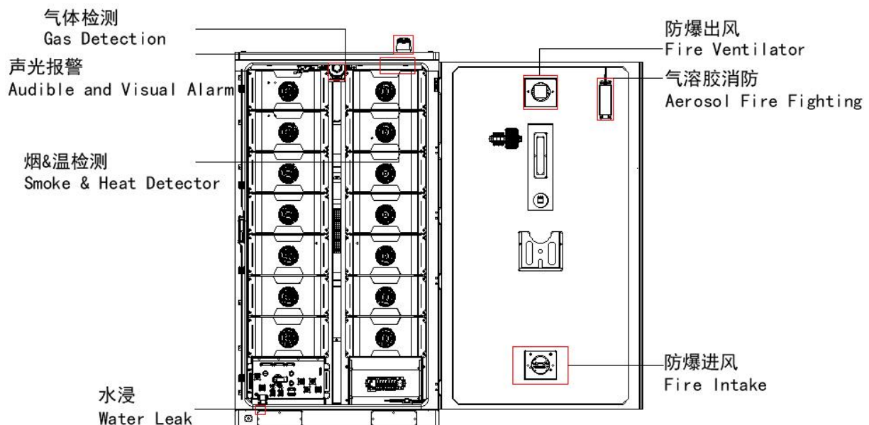
Figure 8.1 Schematic diagram of battery cabinet fire protection system installation
