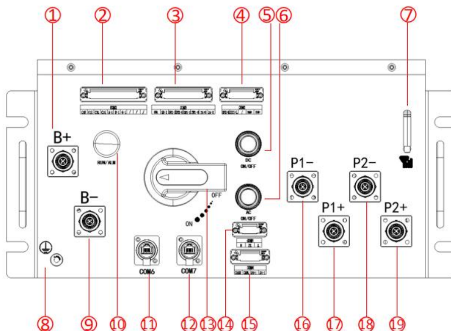
Figure 2.5.3 PDU Description
