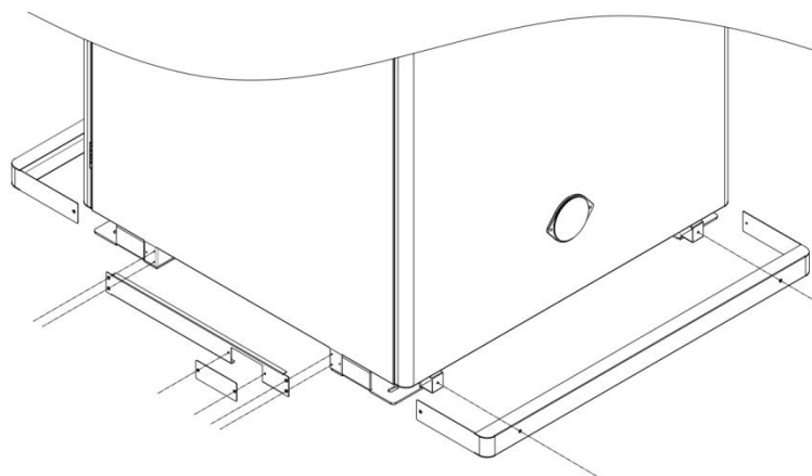
Figure 5.1.1 Schematic diagram of bottom baffle assembly and disassembly
