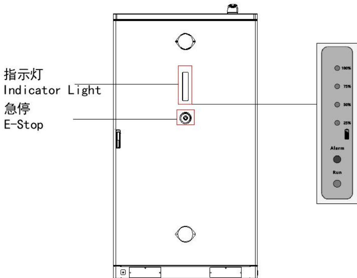
Figure 2.5.5 Indicator Panel Introduction
