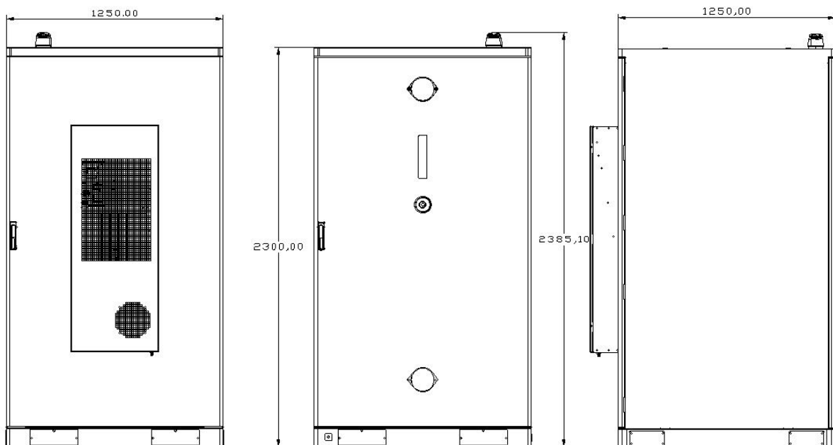
Figure 2.4.1 Product Dimension
