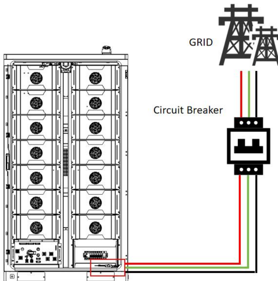
Figure 6.5 Schematic diagram of auxiliary power supply connection
