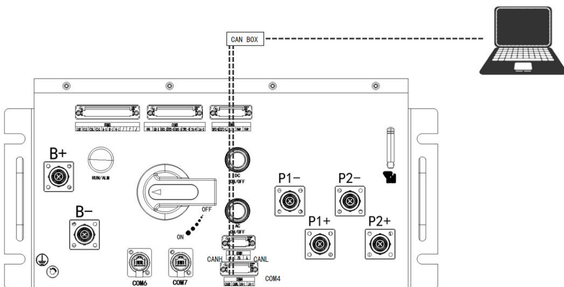
Figure 2.7.1 CAN BOX Connection
