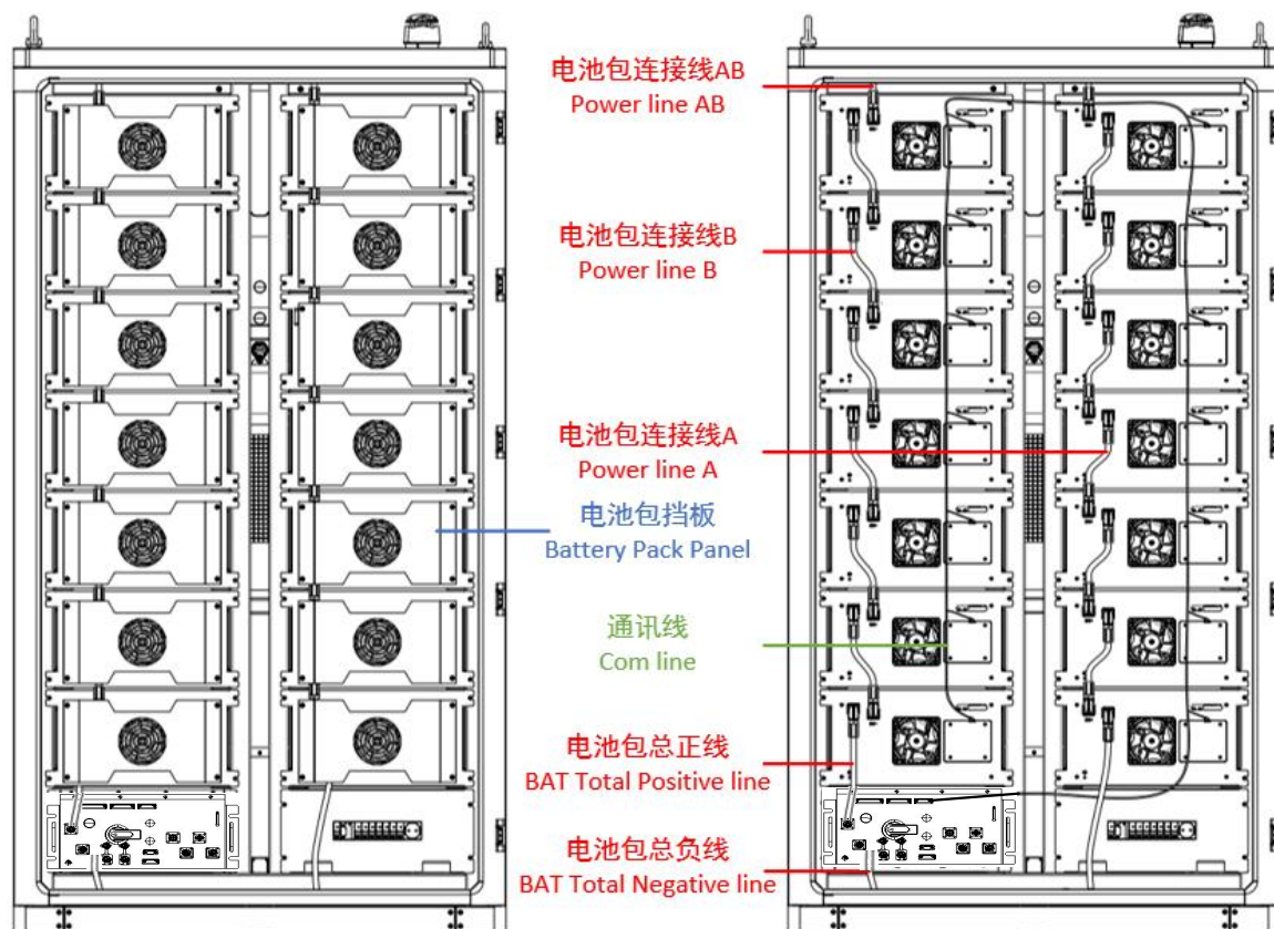
Figure 6.4 Schematic diagram of wire harness installation
