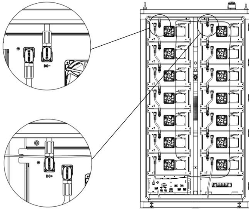
Figure 6.4 Schematic diagram of battery pack installation across connecting wires
