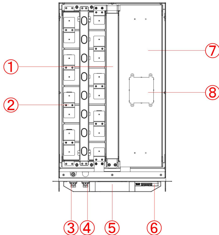
Figure 2.5.1 Battery Pack Design
