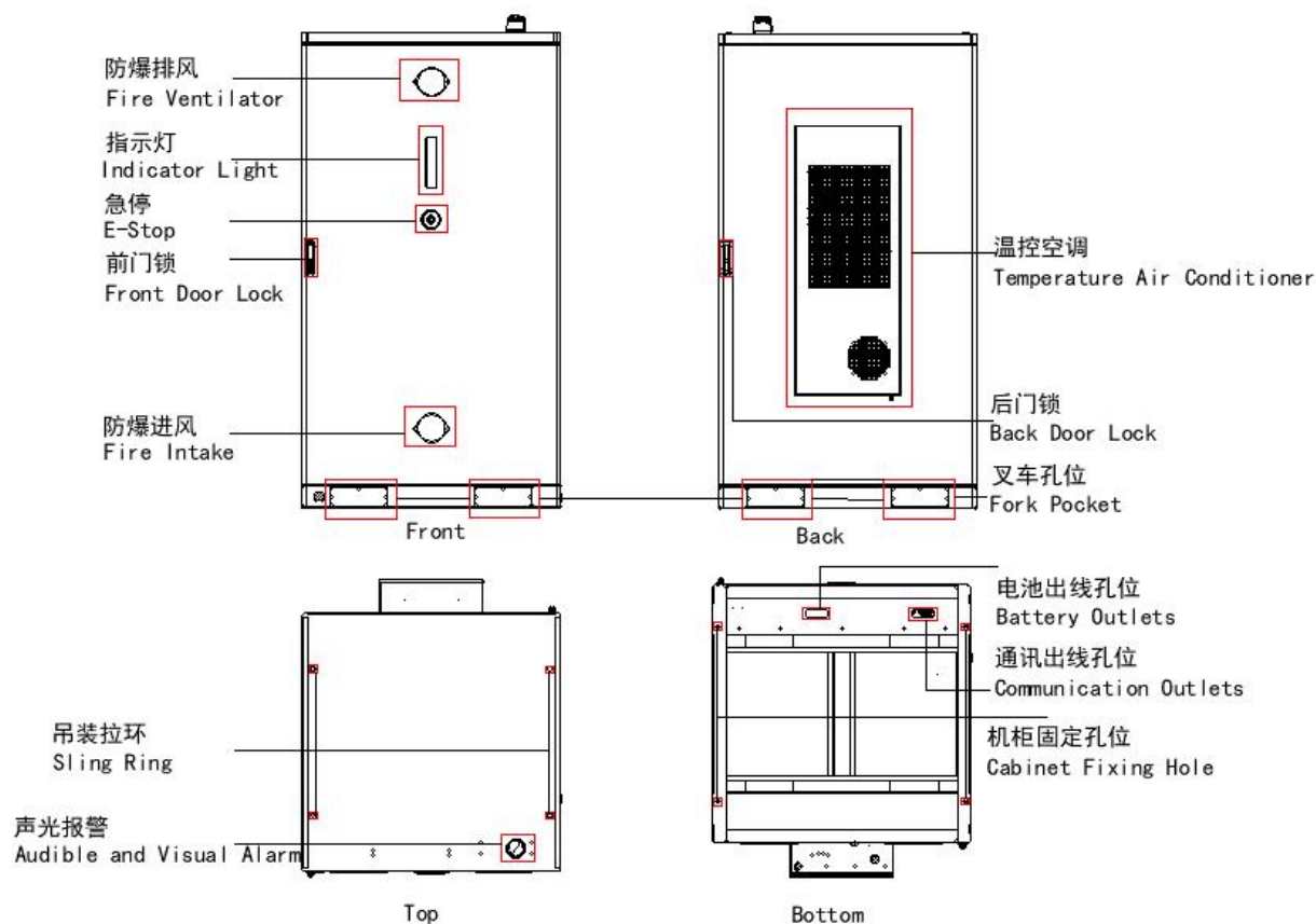
Figure 2.4.2 Product Layout - External
