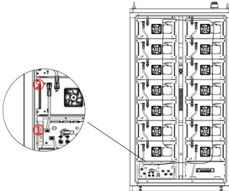
Figure 6.4 Schematic diagram of the main positive connection wire installation of the battery pack
