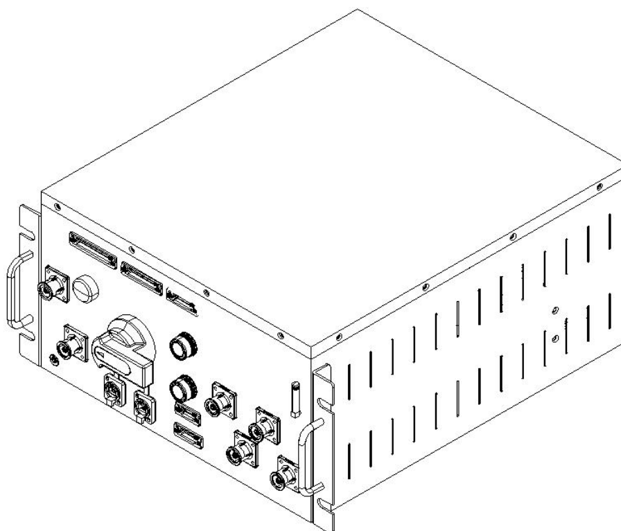
Figure 2.5.3 PDU
