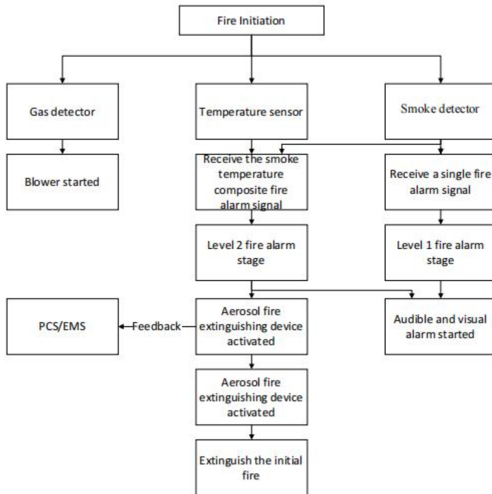
Figure 8.2 Working principle of fire protection system
