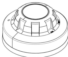
Figure 8.6 Schematic diagram of a smoke sensor
