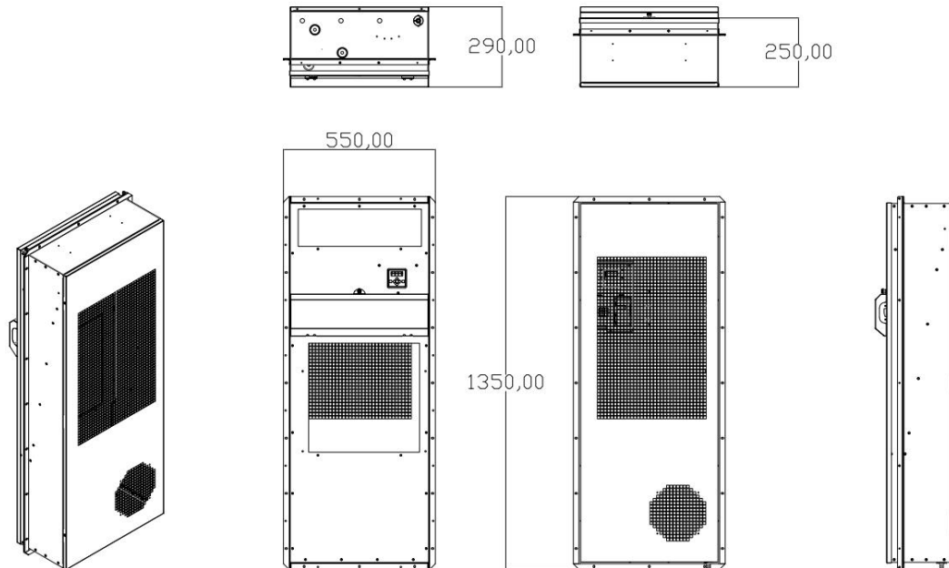
Figure 2.5.4 Industrial Air Conditioner Dimensions
