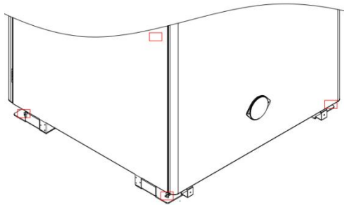
Figure 5.6 Schematic diagram of equipment fixing
