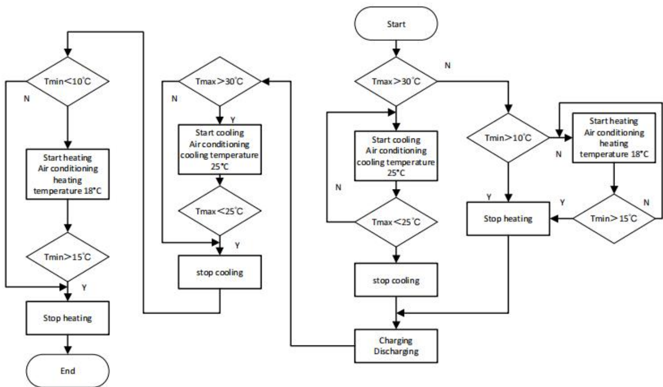
Figure 2.5.4 Industrial air conditioning control logic flow
