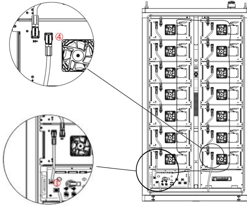
Figure 6.4 Schematic diagram of battery pack main negative connection installation
