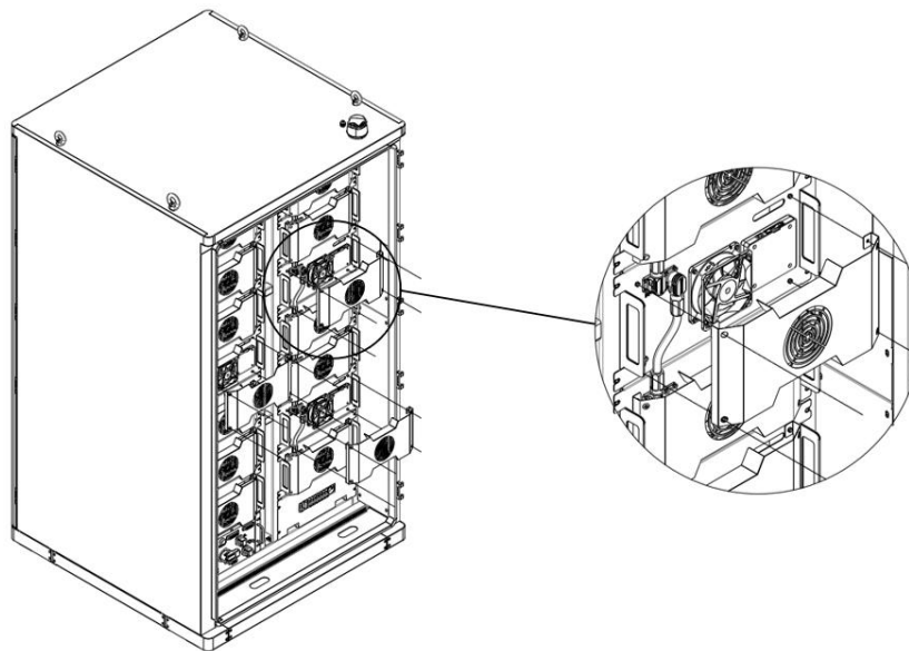
Figure 6.4 Schematic diagram of battery pack panel disassembly and assembly
