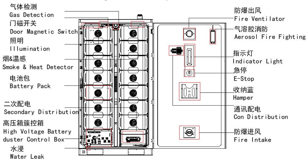
Figure 2.4.2 Product Layout - Internal
