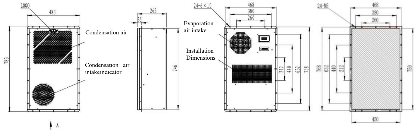
Installation Dimensions
