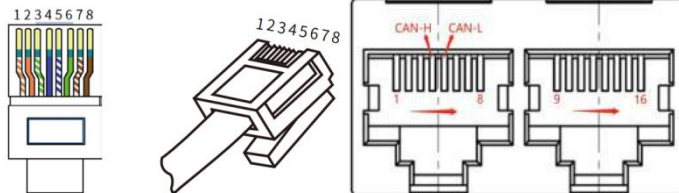
RJ45 Registered Jack
